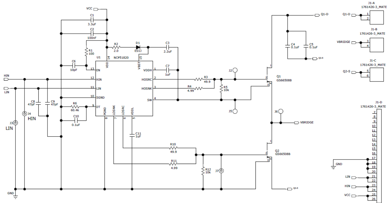
Figure 25. Daughter Card
