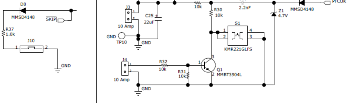
Figure 12. NCP1680 EVB Skip Interfaces
