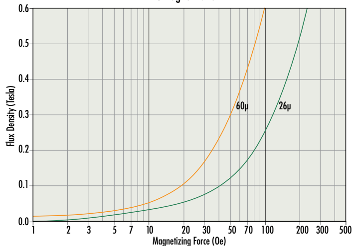
DC Magnetization
